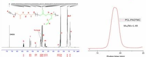
Figures 13 and 14. 1 H NMR and GPC spectra of the obtained polycarbonate-polyester copolymer that will be used for production of polycarbonate "brush"
