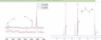
Figures 21 and 22. Raman spectroscopy and 1 H NMR spectrum of the obtained azide-functionalized low-molecular-weight linker.
