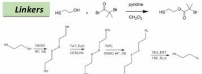
Figures 19 and 20. Reaction scheme for the synthesis of linkers that will be used for functionalization of the cyclic "brush" polymer
