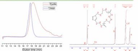
Figures 7 and 8. Gel permeation chromatogram and 1 H NMR spectrum of the obtained cyclized polycaprolactone.
