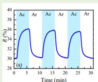
Reflectance measured at a wavelength of 342 nm for copolymer film CP4 within 3 cycles of absorption and desorption of acetone vapors.
